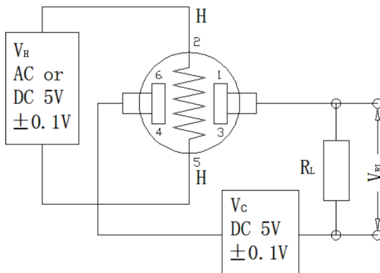
Fig2. MQ-7B Test Circuit
