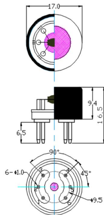
Fig1.Sensor Structure Unit: mm Tolerance: \pm 0.1\text{mm}
