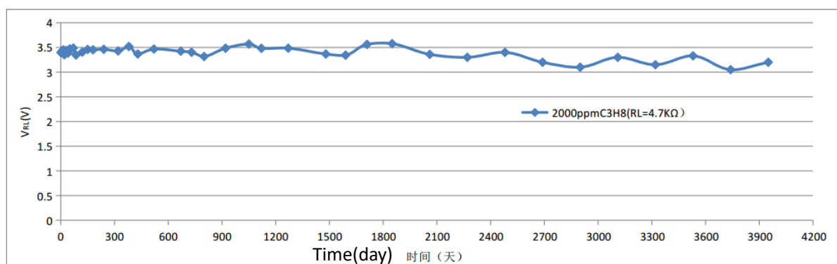
Fig7.long-term Stability
