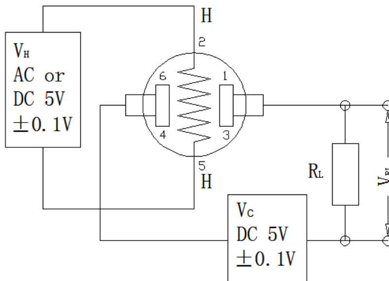
Fig2. MQ-6B Test Circuit
