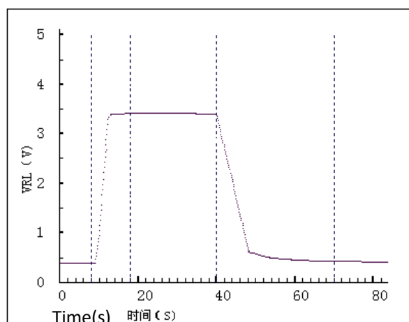
Fig6.Response and Resume
