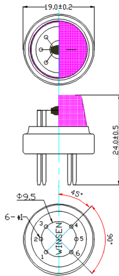
Fig1.Sensor Structure
