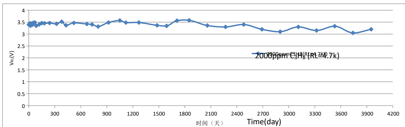
Fig7.long-term Stability
