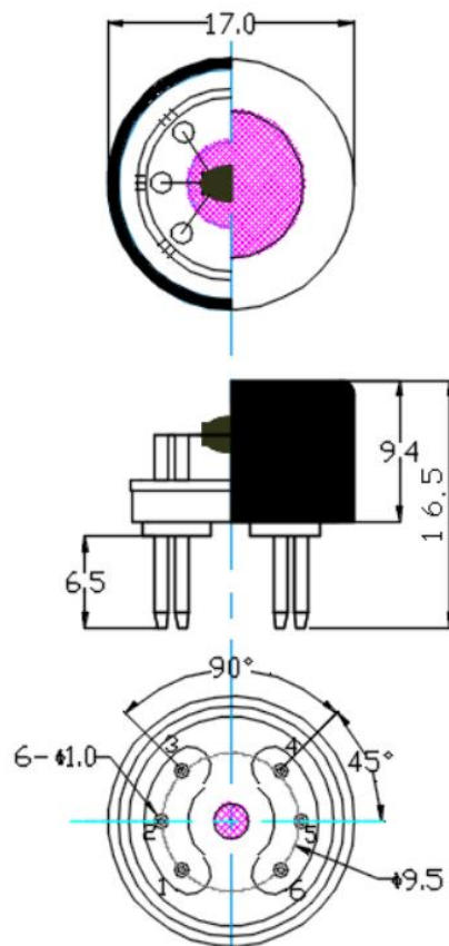
Fig1.Sensor Structure
