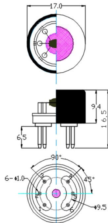
Fig1.Sensor Structure
