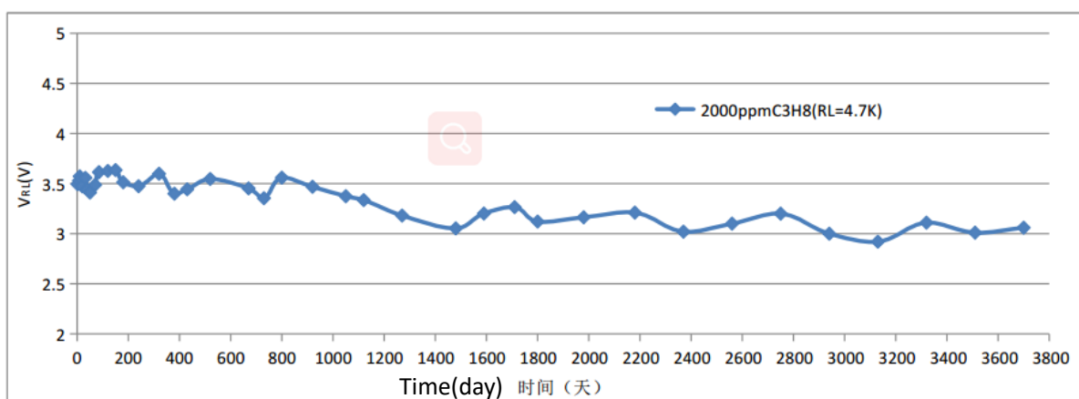
Fig7.long-term Stability
