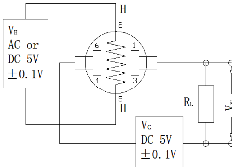
Fig2. MQ-2B Test Circuit
