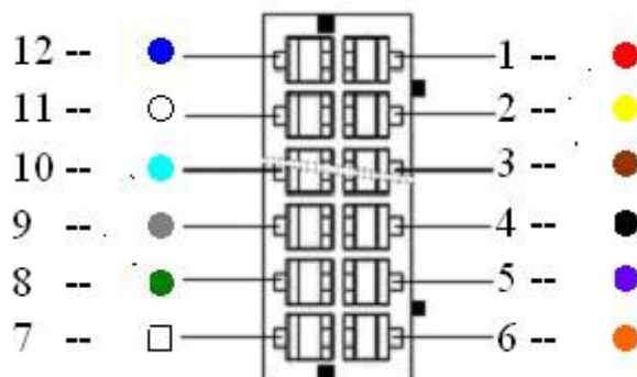
Figure 2 Pin Definition
