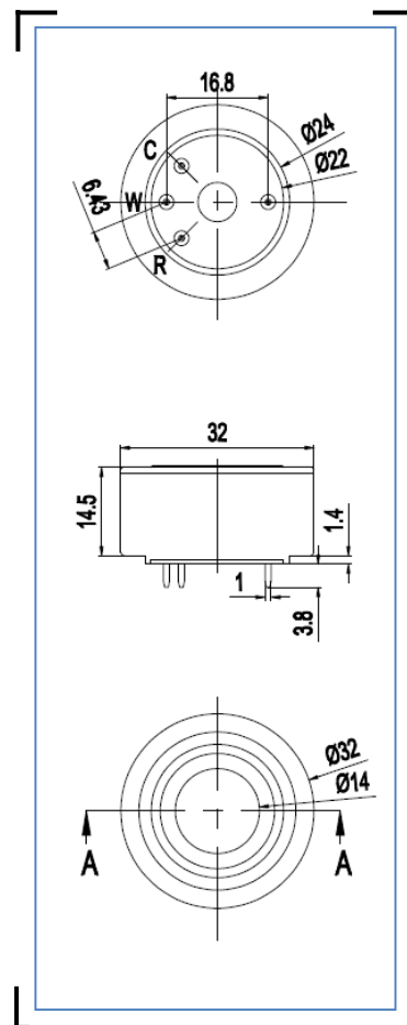
Fig1.Sensor Structure
