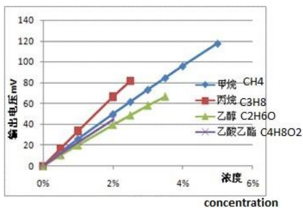
Fig3. Sensitivity Curve
