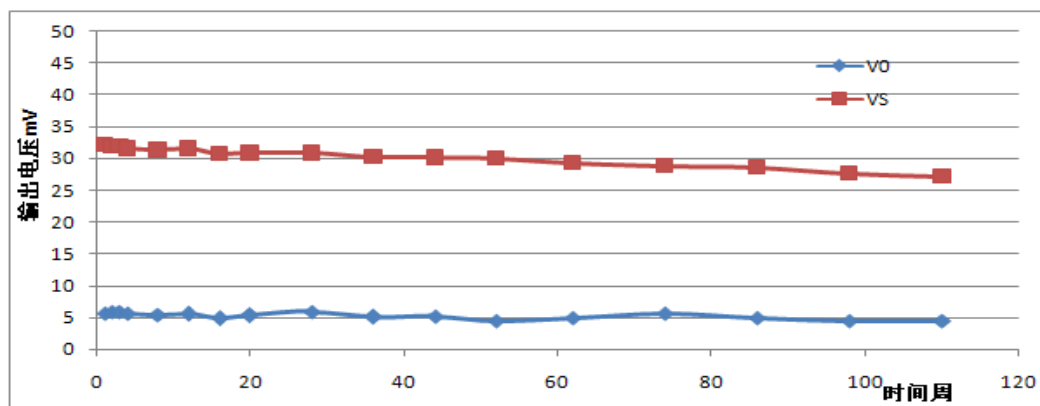
Fig11.Zero and Sensitivity fluctuation
