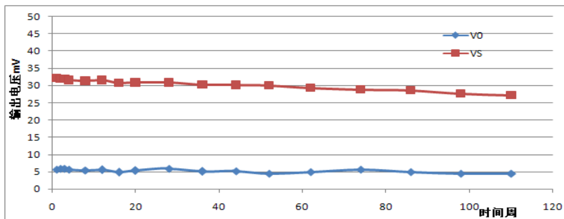
Fig11. Stability of Zero point and Sensitivity
