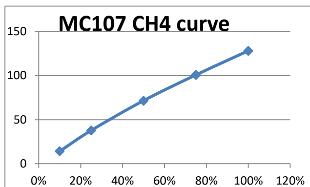
Fig3.Sensitivity Curve
