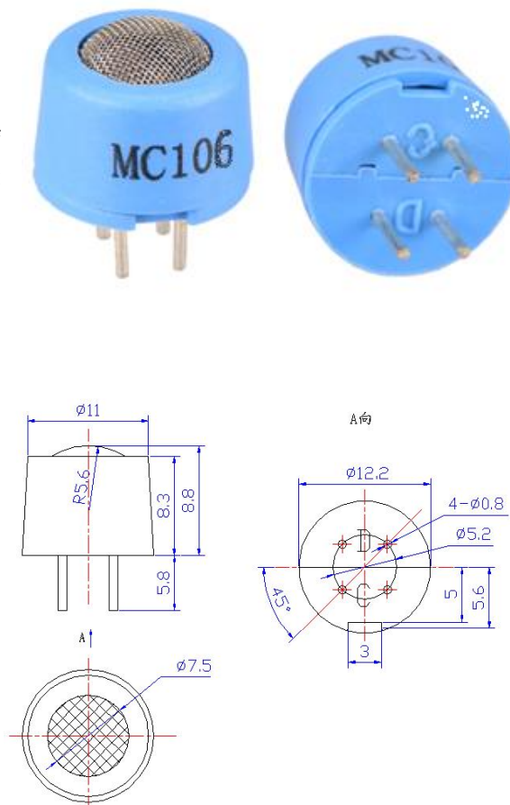
Fig1. Sensor Structure
