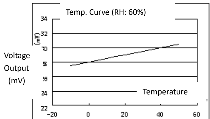
Fig6. Sensitivity at different temp.
