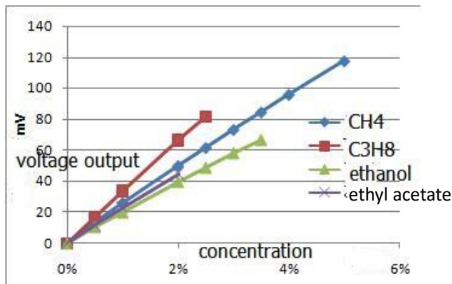
Fig3. Sensitivity Curve
