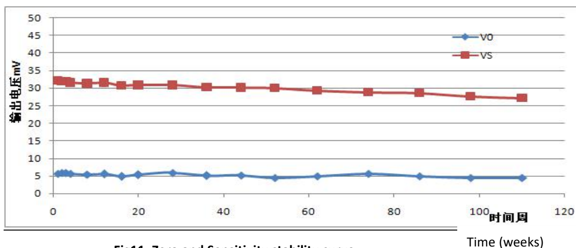
Fig11. Zero and Sensitivity stability curve
